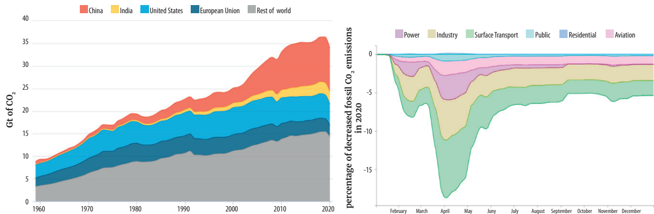
Figure 1: Fossil emissions in Gt for main pollutants (left); drop of fossil emissions during pandemic year 2020 (right)
